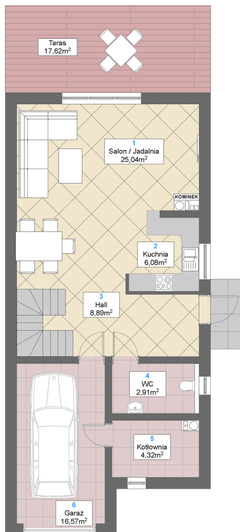
PARTER 63,81m 2
